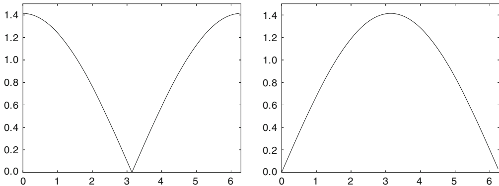
Fig. 5.4 The frequency responses \lambda_{G_0}(\omega) and \lambda_{G_1}(\omega) for the Haar wavelet
