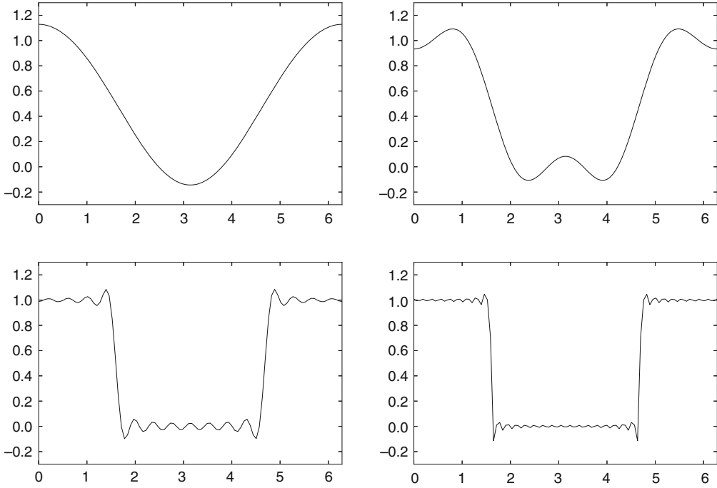
Fig. 3.6 The frequency response which results by including the first 1/32, the first 1/16, the first 1/4, and all of the filter coefficients for the ideal low-pass filter
