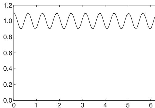
Fig. 3.2 The frequency response of a filter which adds an echo with damping factor c = 0.1 and delay d = 10
