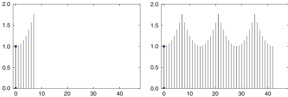
Fig. 5.7 A vector and its symmetric extension. The period of \check{x} is now 2N - 2 . For the vector in Fig. 2.5 it was 2N
