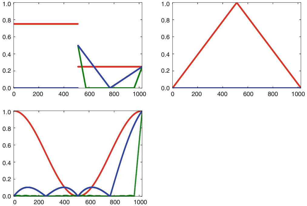
Fig. 4.17 The error (i.e. the contribution from W_0 \oplus W_1 \oplus \dots \oplus W_{m-1} ) for N = 1025 when f is a square wave, the linear function f(t) = 1 - 2|1/2 - t/N| , and the trigonometric function f(t) = 1/2 + \cos(2\pi t/N)/2 , respectively. The detail is indicated for m = 6 and m = 8
