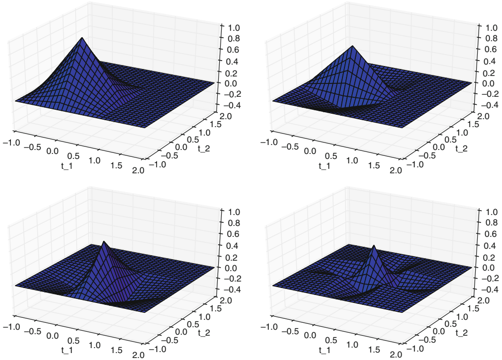
Fig. 9.2 The functions \phi \otimes \phi , \phi \otimes \psi , \psi \otimes \phi , \psi \otimes \psi , which are bases for (V_0 \otimes V_0) \oplus W_0^{(0,1)} \oplus W_0^{(1,0)} \oplus W_0^{(1,1)} for the alternative piecewise linear wavelet
