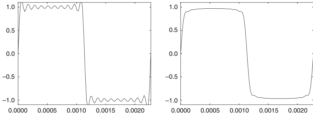
Fig. 1.12 f_N(t) and S_N(t) for N = 20
