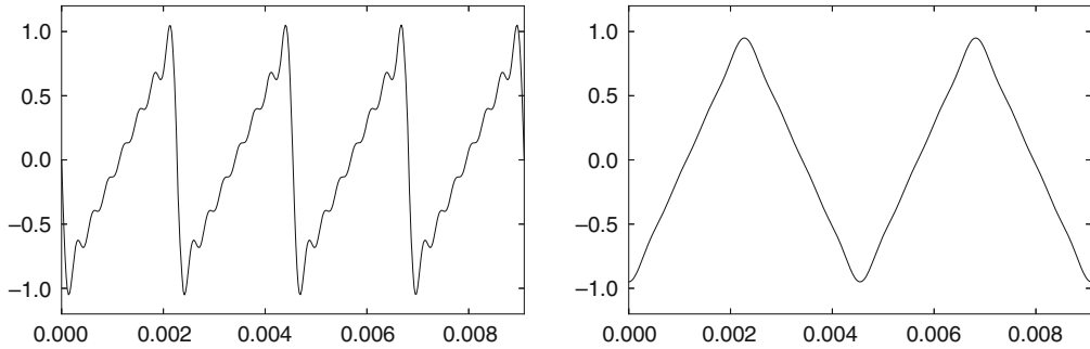
Fig. 1.11 The Fourier series with N = 7 terms of the periodic- (left) and symmetric (right) extensions of the function in Example 1.36
