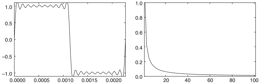
Fig. 1.6 The Fourier series of the square wave with N = 20 , and the values for the first 100 Fourier coefficients b_n
