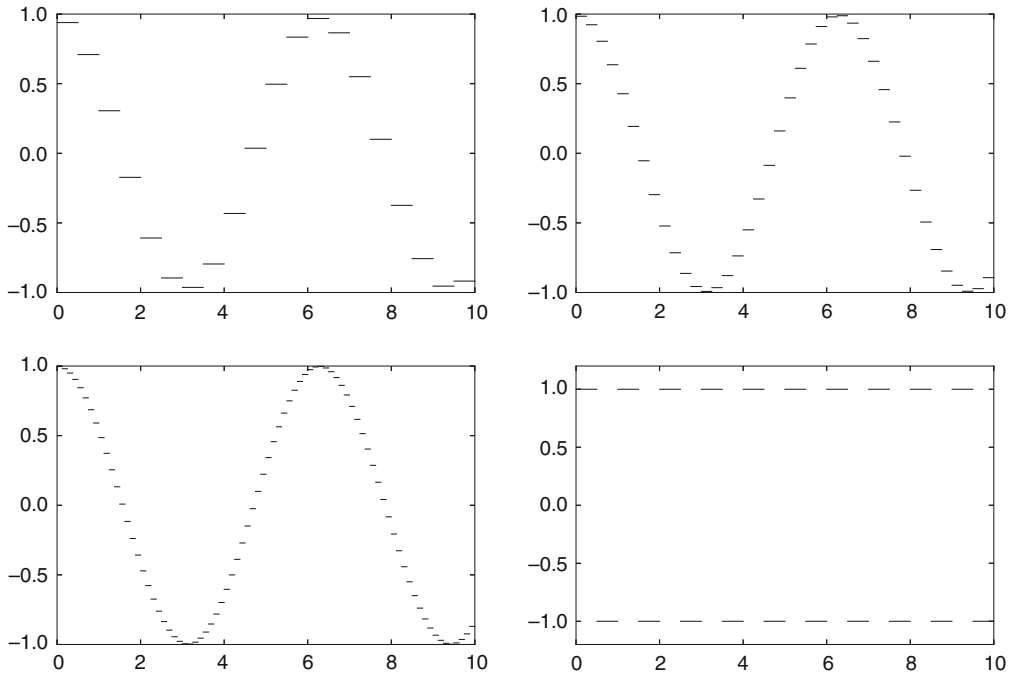
Fig. 4.5 Piecewise constant approximations to \cos t on the interval [0, 10] in the spaces V_1, V_2 , and V_3 . The lower right plot shows the square wave in V_2
