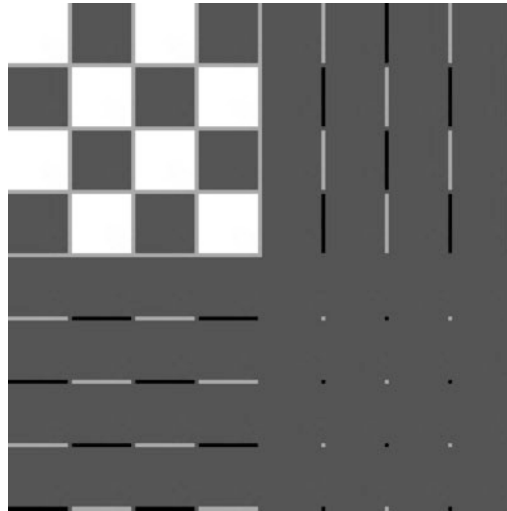
Fig. 9.6 The chess pattern example image after application of the 2D DWT. The Haar wavelet was used
