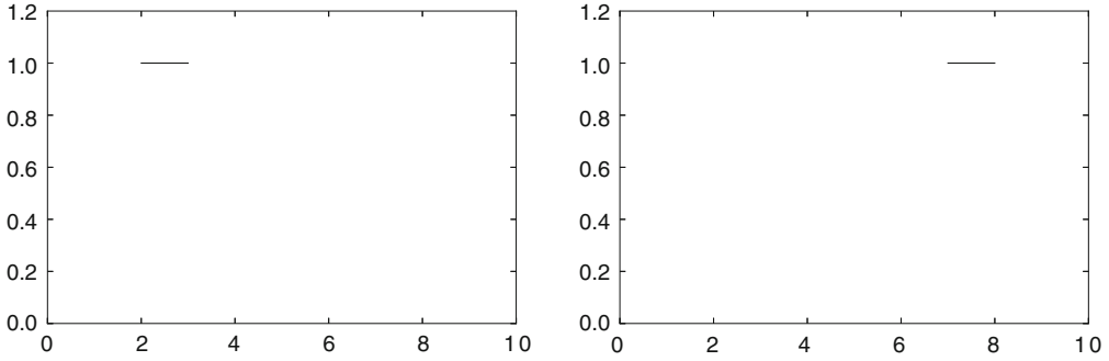
Fig. 4.3 The basis functions \phi_2 and \phi_7 from \phi_0
