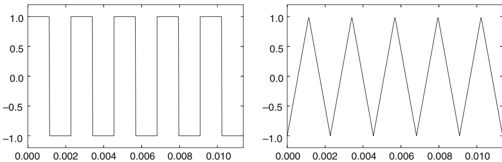
Fig. 1.4 The first five periods of the square wave and the triangle wave
