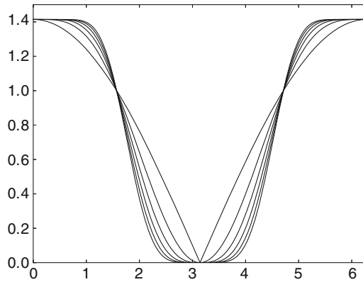
Fig. 6.3 The magnitudes |\lambda_{G_0}(\omega)| = |\lambda_{H_0}(\omega)| for the first orthonormal wavelets
