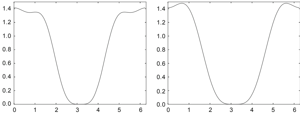
Fig. 6.1 The frequency responses \lambda_{H_0}(\omega) (left) and \lambda_{G_0}(\omega) (right) for the CDF 9/7 wavelet
