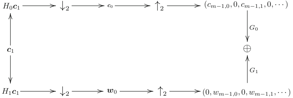
Fig. 5.3 Detailed illustration of DWT and IDWT
