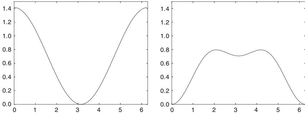
Fig. 5.5 The frequency responses \lambda_{G_0}(\omega) and \lambda_{G_1}(\omega) for the alternative piecewise linear wavelet
