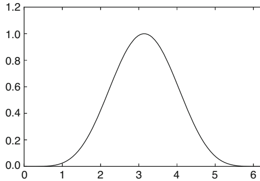
Fig. 3.9 The frequency response of the high-pass filter deduced from row 5 of Pascal's triangle
