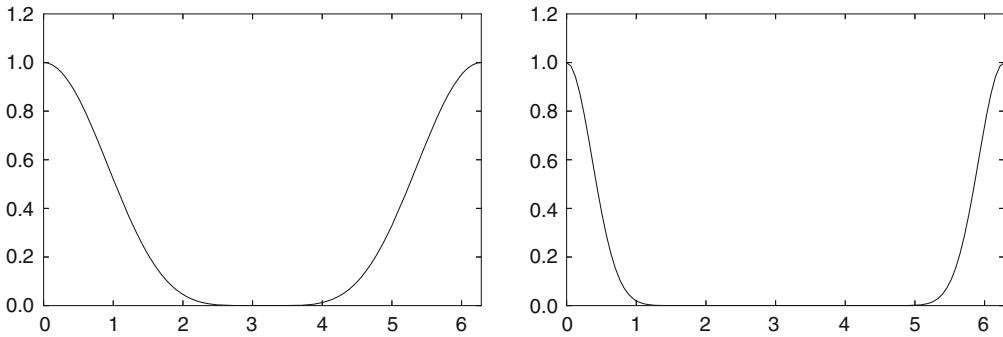
Fig. 3.8 The frequency response of filters corresponding to iterating the moving average filter \{1/2, 1/2\} k = 5 and k = 30 times (i.e. using row k in Pascal's triangle)
