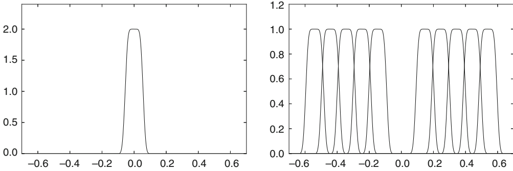
Fig. 3.7 Frequency responses of some filters used in the MP3 standard (right). They are simply shifts of that of the prototype filter (left)
