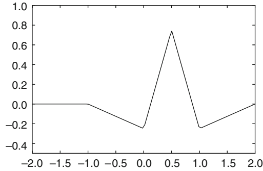
Fig. 4.18 The function \hat{\psi} we constructed as an alternative wavelet for piecewise linear functions
