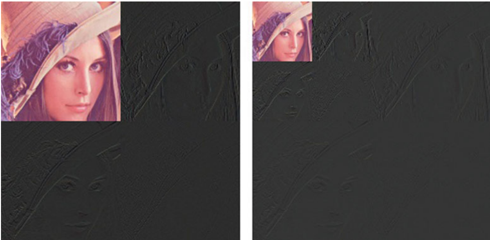
Fig. 9.8 The corresponding image resulting from a wavelet transform with the Haar-wavelet for m = 1 and m = 2
