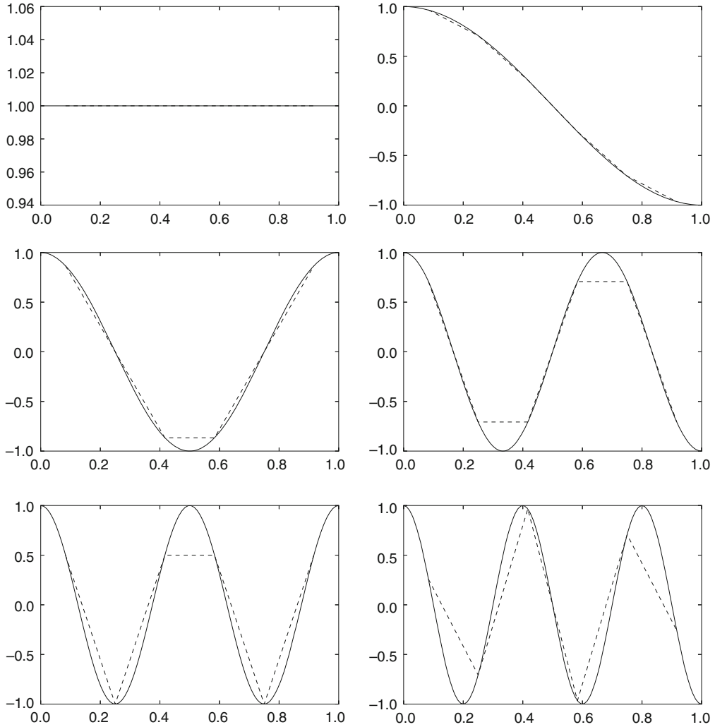
Fig. 2.6 The six different sinusoids used in DCT for N = 6 , i.e. \cos(2\pi nt/2) , 0 \leq n < 6 . The plots also show piecewise linear functions (dashed lines) between the sample points \frac{2k+1}{2N} , 0 \leq k < 6
