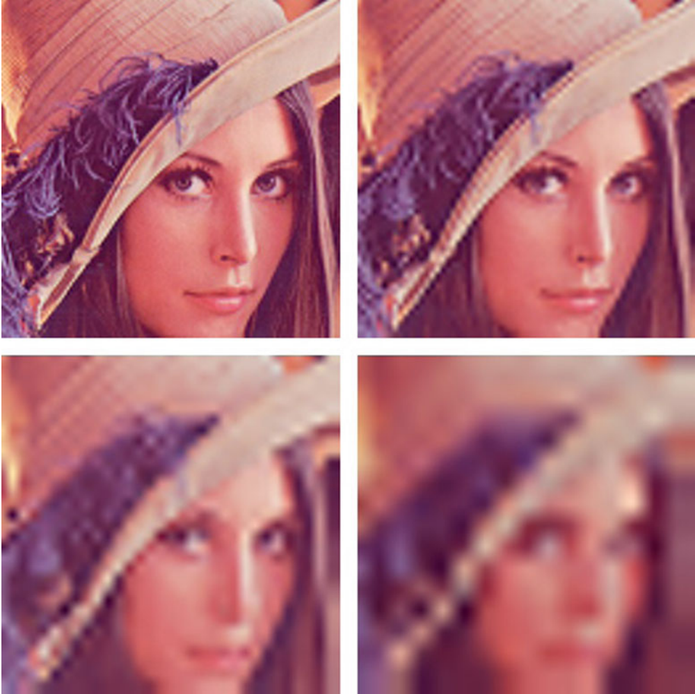
Fig. 9.11 Low resolution approximations of the Lena image, for the CDF 9/7 wavelet
