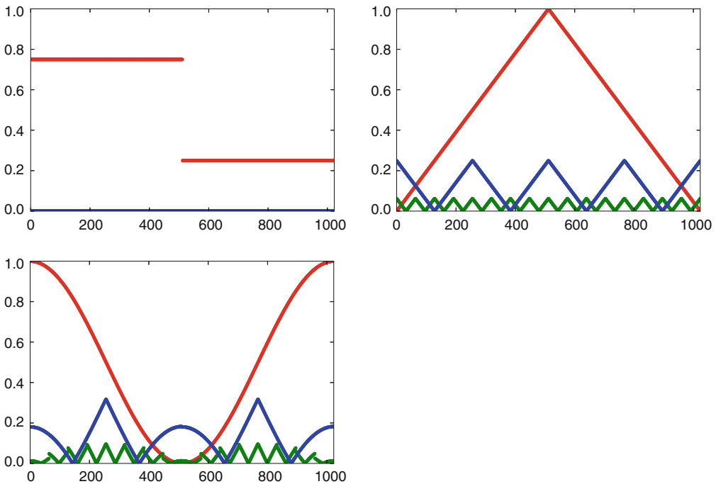
Fig. 4.12 The error in a 1024-point DWT of the samples of three functions (red): a square wave, the linear function f(t) = 1 - 2|1/2 - t/N| , and the trigonometric function f(t) = 1/2 + \cos(2\pi t/N)/2 . The detail is indicated for m = 6 (green) and m = 8 (blue)
