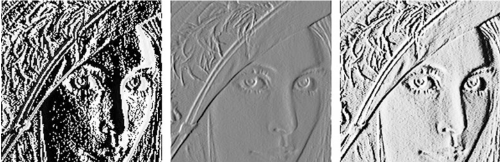
Fig. 8.11 Experimenting with the partial derivative in the x -direction for the image in Fig. 8.4. The left image has artifacts, since the pixel values are outside the legal range. We therefore normalize the intensities to lie in [0, 255] (middle), before we increase the contrast (right)
