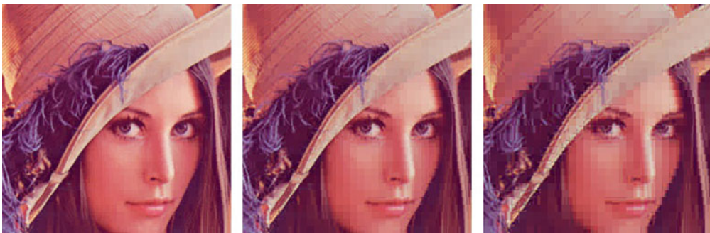
Fig. 8.17 The effect on an image when it is transformed with the DFT, and the DFT-coefficients below a certain threshold are zeroed out. The threshold has been increased from left to right, from 100, to 200, and 400. The percentage of pixel values that were zeroed out are 76.6, 89.3, and 95.3, respectively
