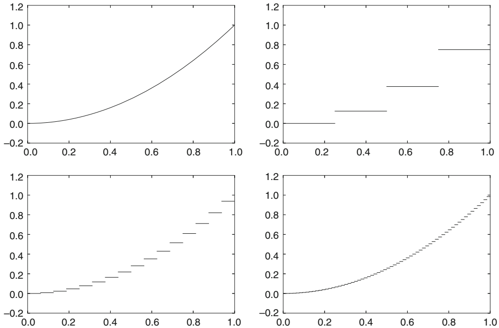
Fig. 4.6 Comparison of the function defined by f(t) = t^2 on [0, 1] with the projection onto V_2 , V_4 , and V_6 , respectively
