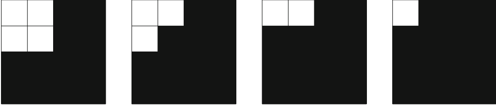
Fig. 9.5 Discarding wavelet coefficients at the second level. After the second stage in the 2D DWT, the coefficients from the upper left corner are also split into four parts (left). In the following figures we have removed coefficients from W_2^{(1,1)} , W_2^{(1,0)} , and W_2^{(0,1)} , respectively
