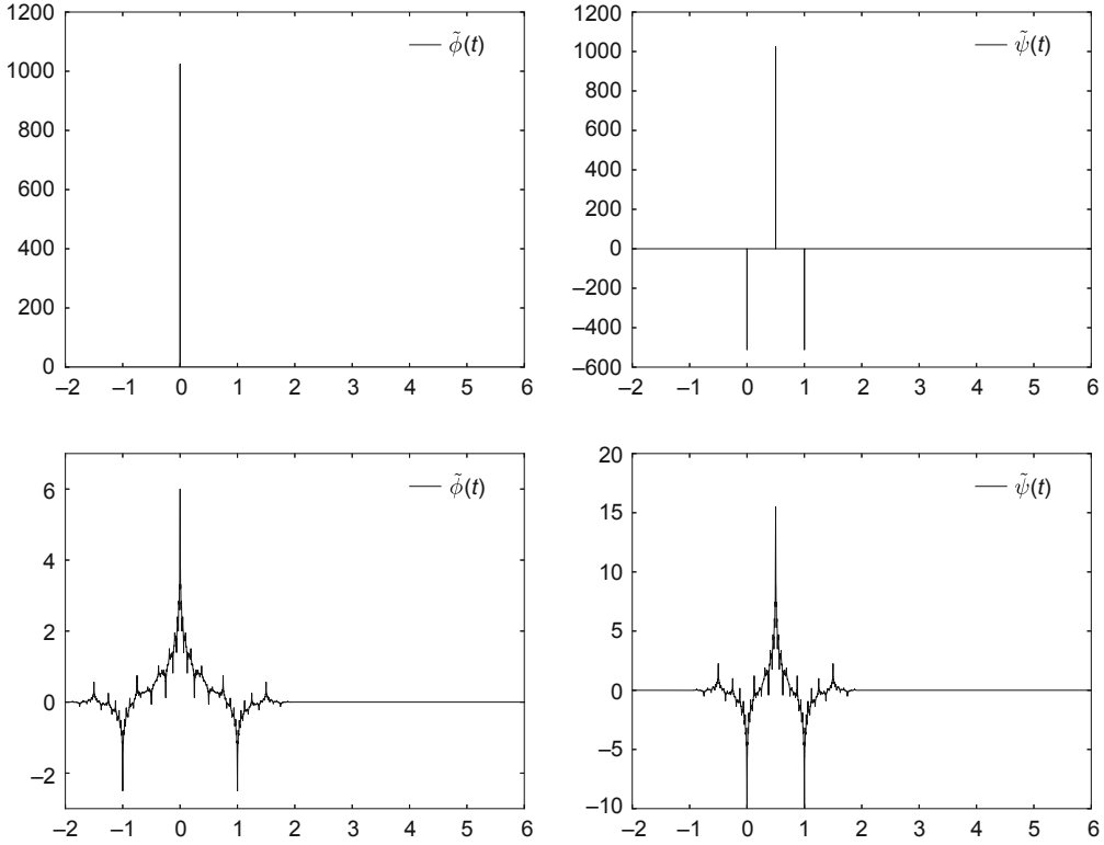
Fig. 5.6 Dual functions for the two piecewise linear wavelets. The functions for the alternative piecewise linear wavelet is shown at the bottom
