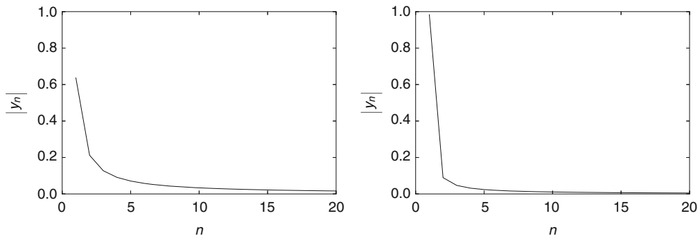
Fig. 1.8 Plot of |y_n| when f(t) = e^{2\pi it/T_2} , and T_2 > T . Left: T/T_2 = 0.5 . Right: T/T_2 = 0.9
