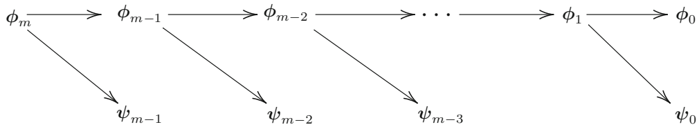
Fig. 4.9 Illustration of a wavelet transform
