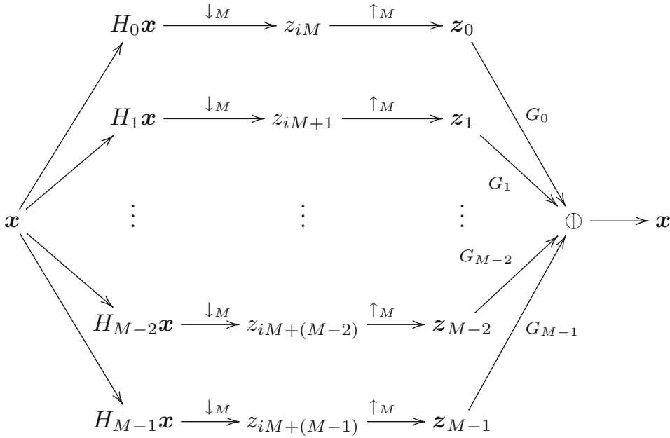
Fig. 5.8 Illustration of forward and reverse filter bank transforms
