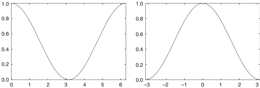
Fig. 3.1 |\lambda_S(\omega)| of the filter from Formula (3.13), plotted over [0, 2\pi] and [-\pi, \pi]
