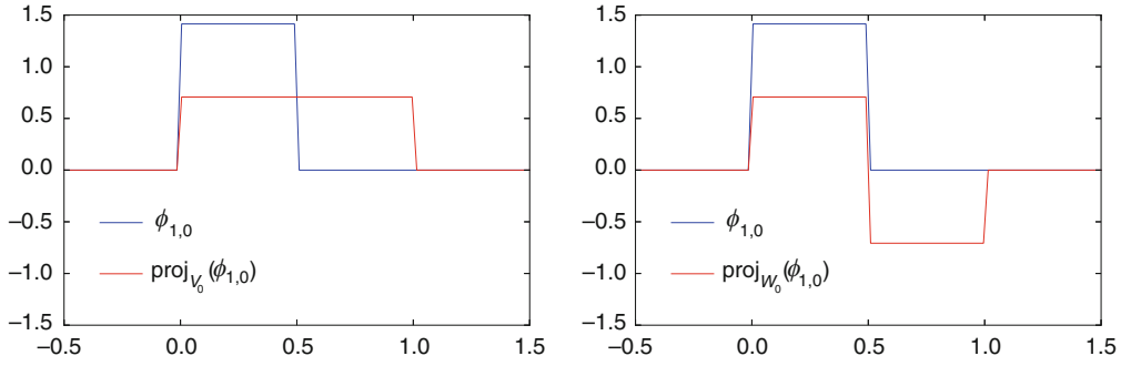
Fig. 4.8 The projection of \phi_{1,0} \in V_1 onto V_0 and W_0
