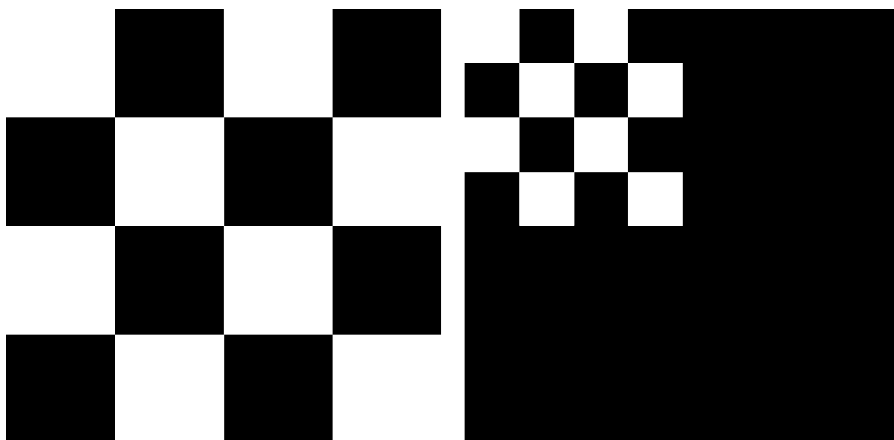
Fig. 9.17 A simple image before and after one level of the 2D DWT. The Haar wavelet was used
