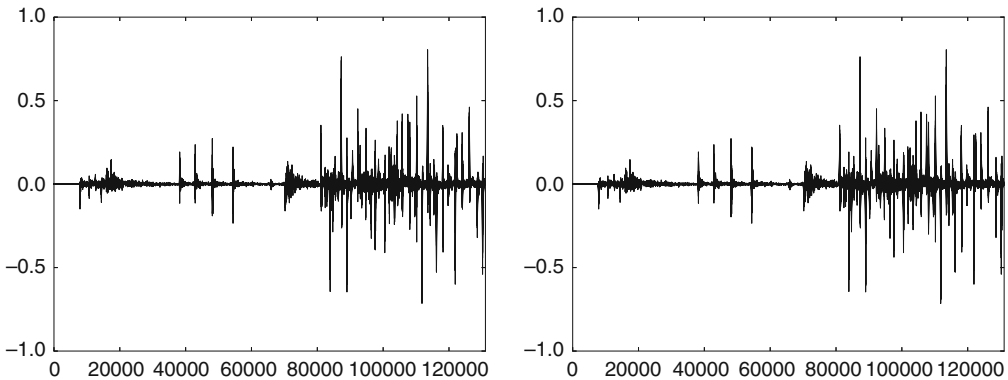
Fig. 4.19 The detail in our audio sample file for the alternative piecewise linear wavelet, for m = 1 (left) and m = 2 (right)
