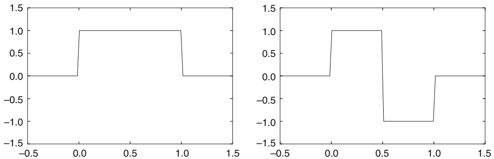
Fig. 4.7 The functions \phi and \psi we used to analyze the space of piecewise constant functions
