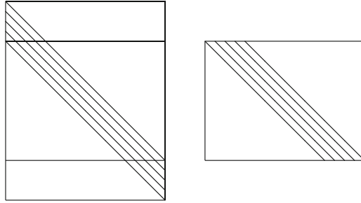
Fig. 3.3 Matrix for the operation \mathbf{x} \rightarrow \mathbf{t} * \mathbf{x} (left), as well as this matrix with the first and last 2L rows dropped (right)
