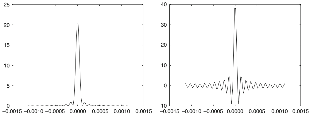
Fig. 1.13 The Fejer and Dirichlet kernels for N = 20
