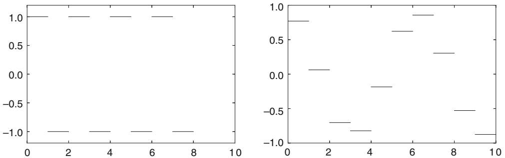
Fig. 4.4 Examples of functions from V_0 . The square wave in V_0 (left), and an approximation to \cos t from V_0 (right)
