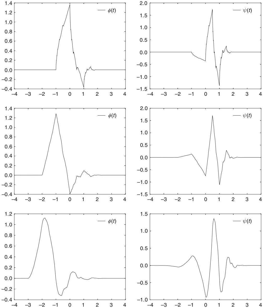
Fig. 6.4 The scaling functions and mother wavelets for orthonormal wavelets with N vanishing moments, for different values of N
