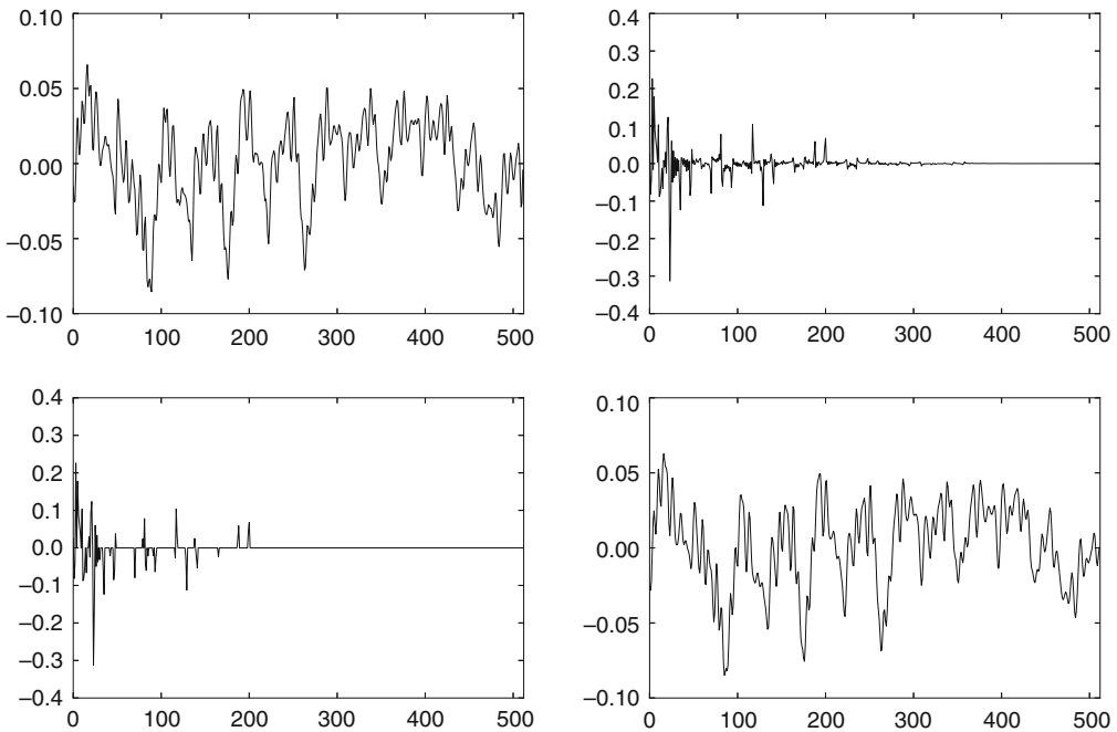
Fig. 2.2 Experimenting with the DFT on a small part of a song
