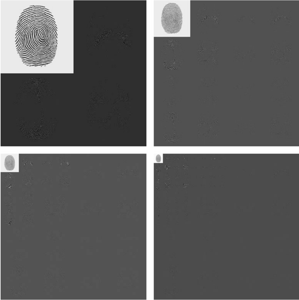
Fig. 9.20 The fingerprint image after several DWT's
