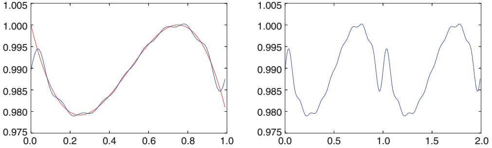
Fig. 1.5 A cubic polynomial on the interval [0, 1] , together with its Fourier series of order 9 (left). The Fourier series on a larger interval is shown right
