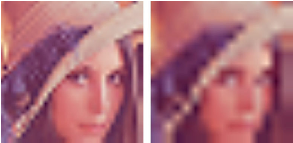
Fig. 9.15 Image of Lena, with detail including level 3 and 4 zeroed out. The Spline 5/3 wavelet was used
