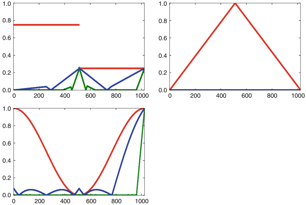
Fig. 4.20 The error (i.e. the contribution from W_0 \oplus W_1 \oplus \dots \oplus W_{m-1} ) for N = 1025 when f is a square wave, the linear function f(t) = 1 - 2|1/2 - t/N| , and the trigonometric function f(t) = 1/2 + \cos(2\pi t/N)/2 , respectively. The detail is indicated for m = 6 and m = 8
