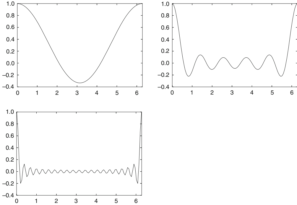
Fig. 3.5 The frequency response of moving average filters with L = 1 , L = 5 , and L = 20
