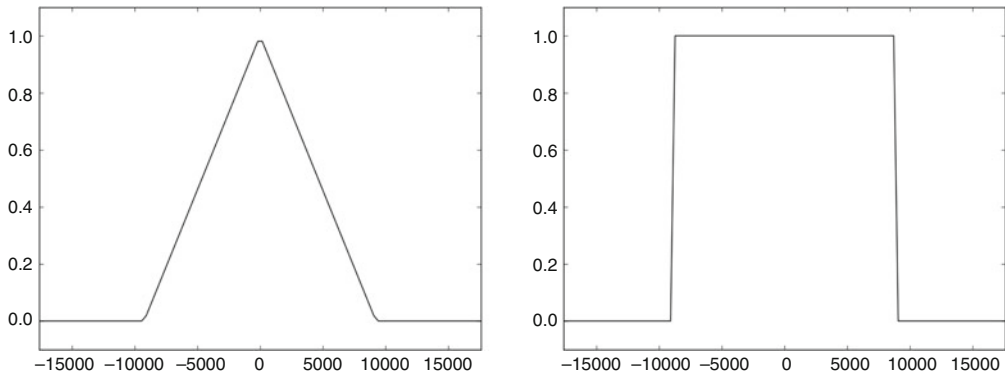
Fig. 1.14 The frequency responses for the filters with Fejer and Dirichlet kernels
