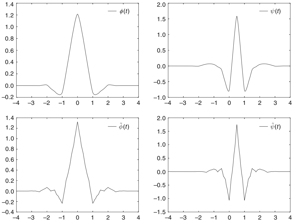
Fig. 6.2 Scaling functions and mother wavelets for the CDF 9/7 wavelet
